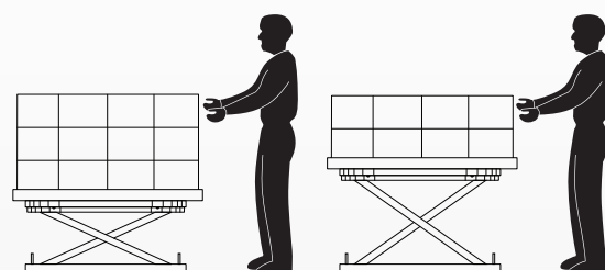
The top layer is maintained in the 750 to 1000 mm recommended ideal work height envelope.
